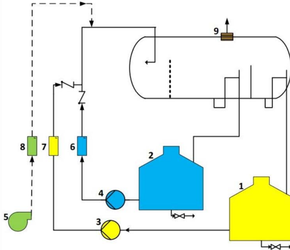
1: Oil tank 2: Water tank 3: Oil pump 4: Water pump 5: Air pump 6: Water flow meter 7: Oil flow meter 8: Air flow meter 9: Mist extractor 10: Non-return valve
