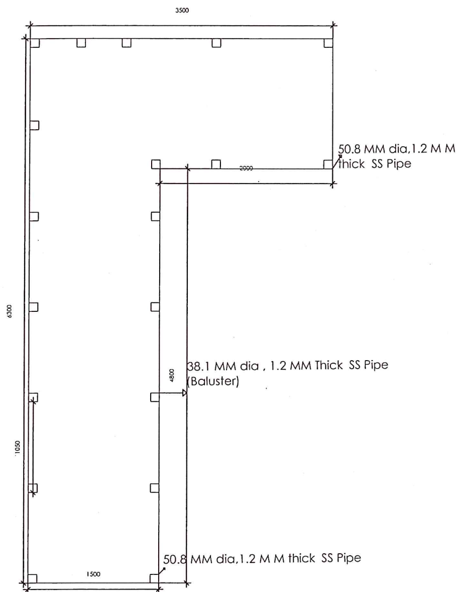
Plan of SS Railing work of Vivekanand Sabhagaar Ramp area
