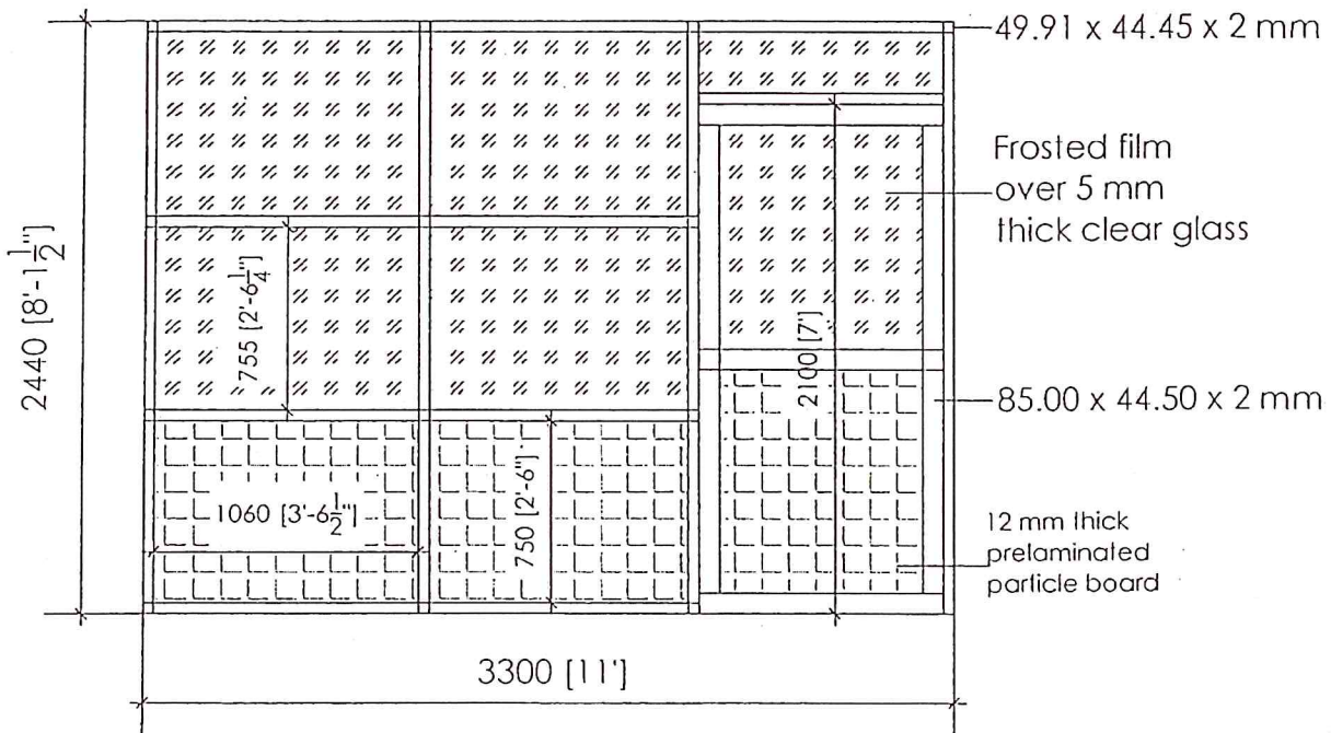
Elevation (A) of Aluminium Partition work
